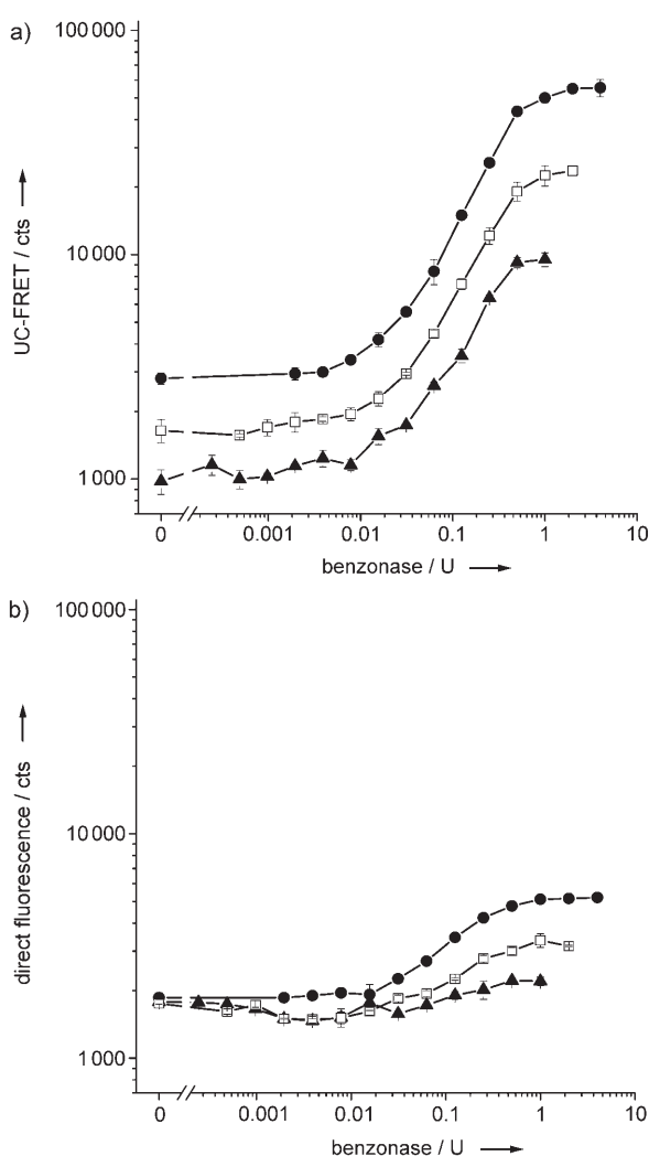
Figure 2. Standard curves of the benzonase-activity assay a) with upconversion or b) without upconversion (conventional method). Emission of the AF680 was measured from buffer by using different amounts of double-labeled substrate oligonucleotide (25 fmol: \blacktriangle ; 50 fmol: \square ; 100 fmol: \bullet ) and optimized quantities of donor UCP particles in the upper figure (25, 50, or 100 ng, respectively). U: activity units; cts: counts.
